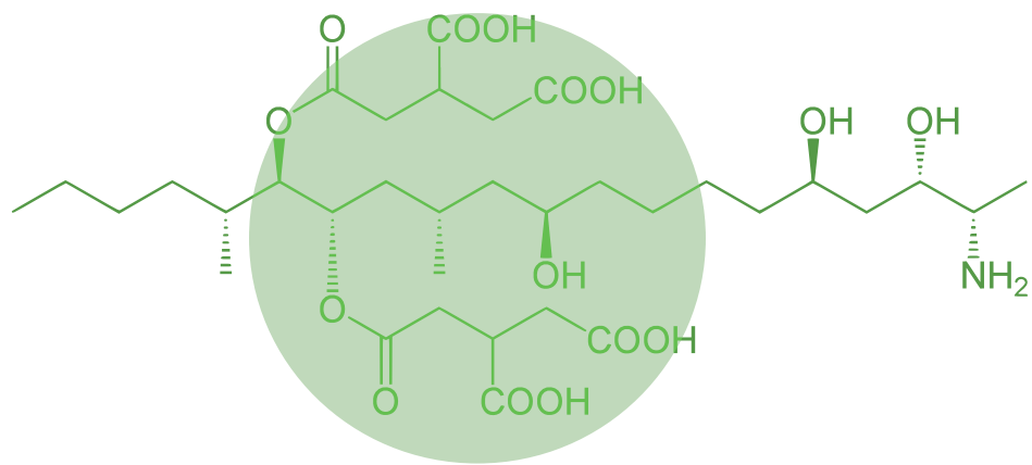
Fumonisin B1/Fumonisina B1
